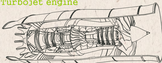
Turbojet engine
